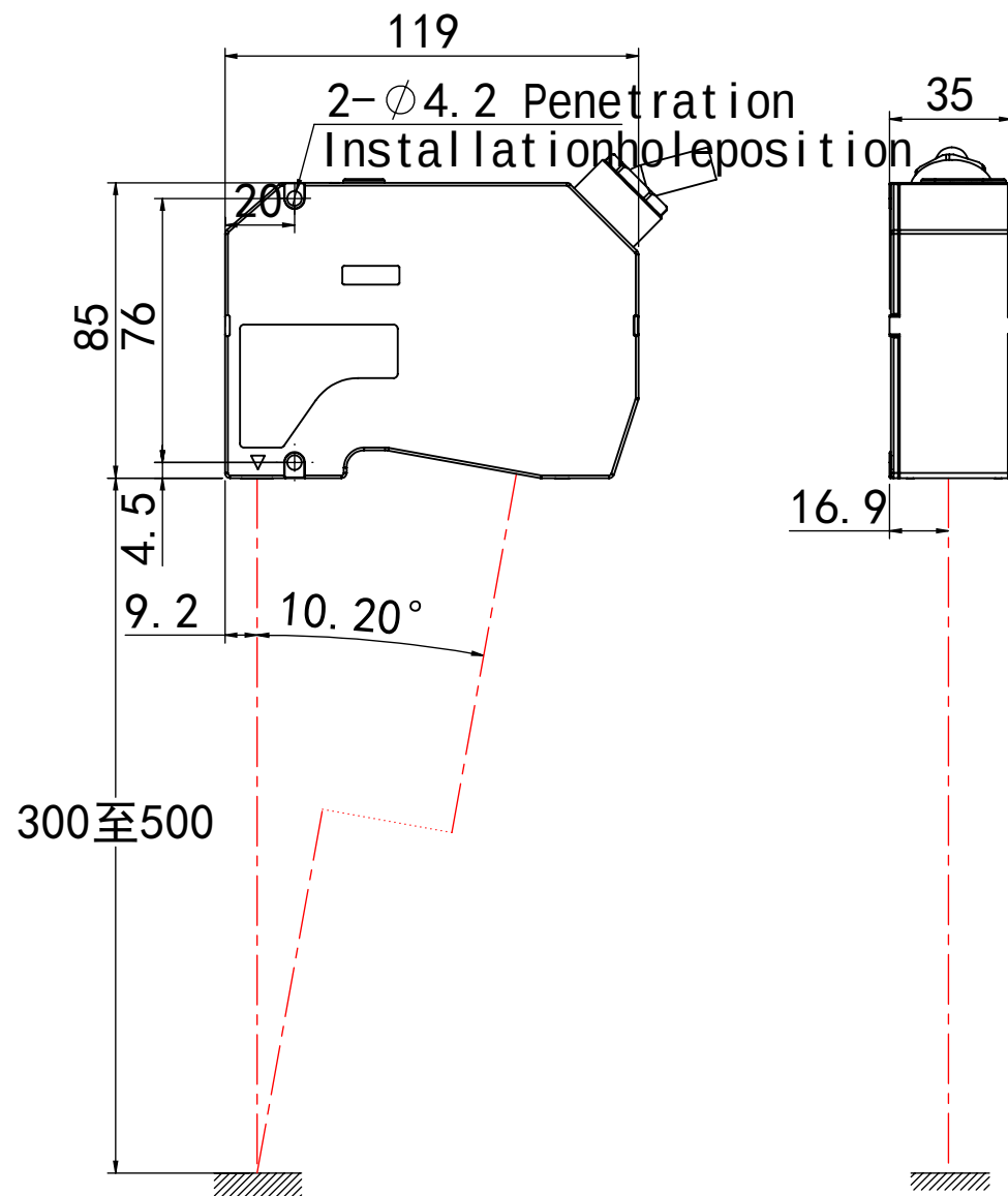
Diffuser reflection installation
